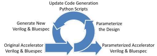
Figure 2: Overview of development workflow.
